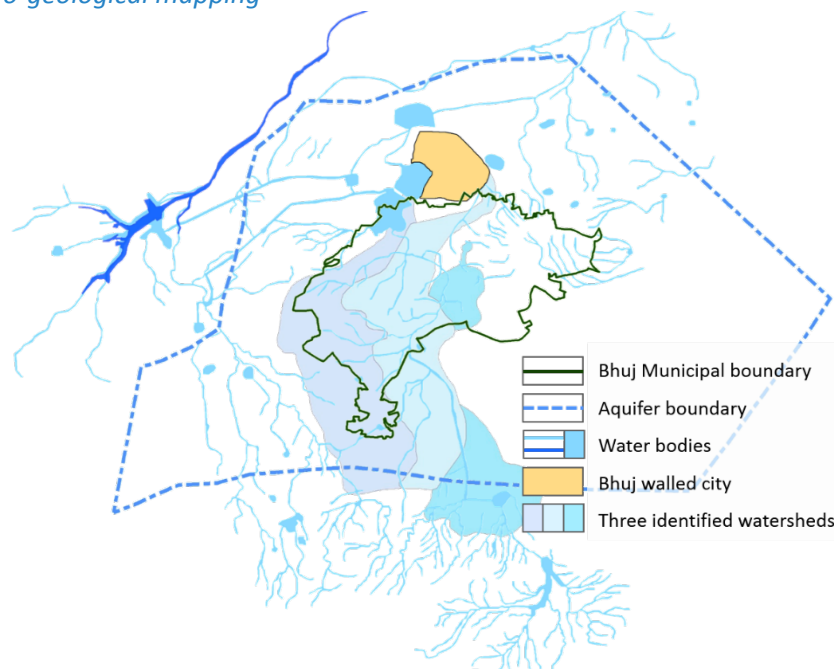
Figure 22: Hydro-geological mapping
