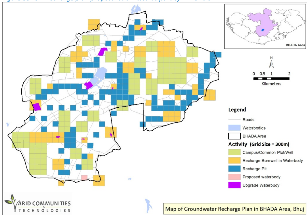
Figure 33: GW recharge plan proposal submitted as part of DP revision
