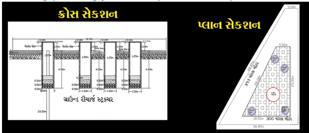
Figure 31: Recharge plot drawings for Jubilee colony – cross section and plan
