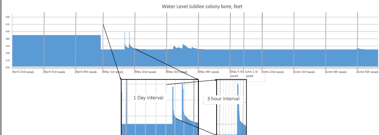
Figure 32: Water level graph for April-June 2016, Jubilee colony recharge borewell
