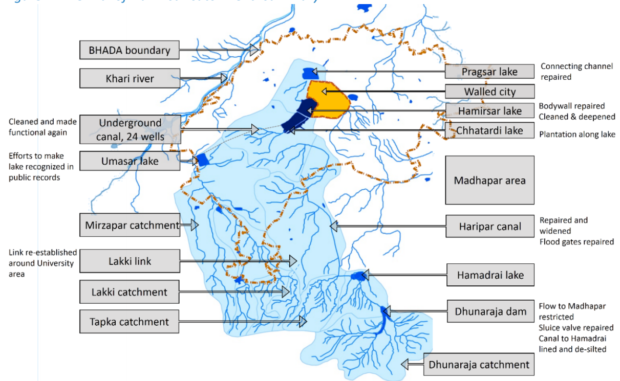
Figure 27: Revival of Hamirsar catchment- summary
