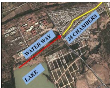
Figure 5: Schematic map of 24 wells over underground channel
