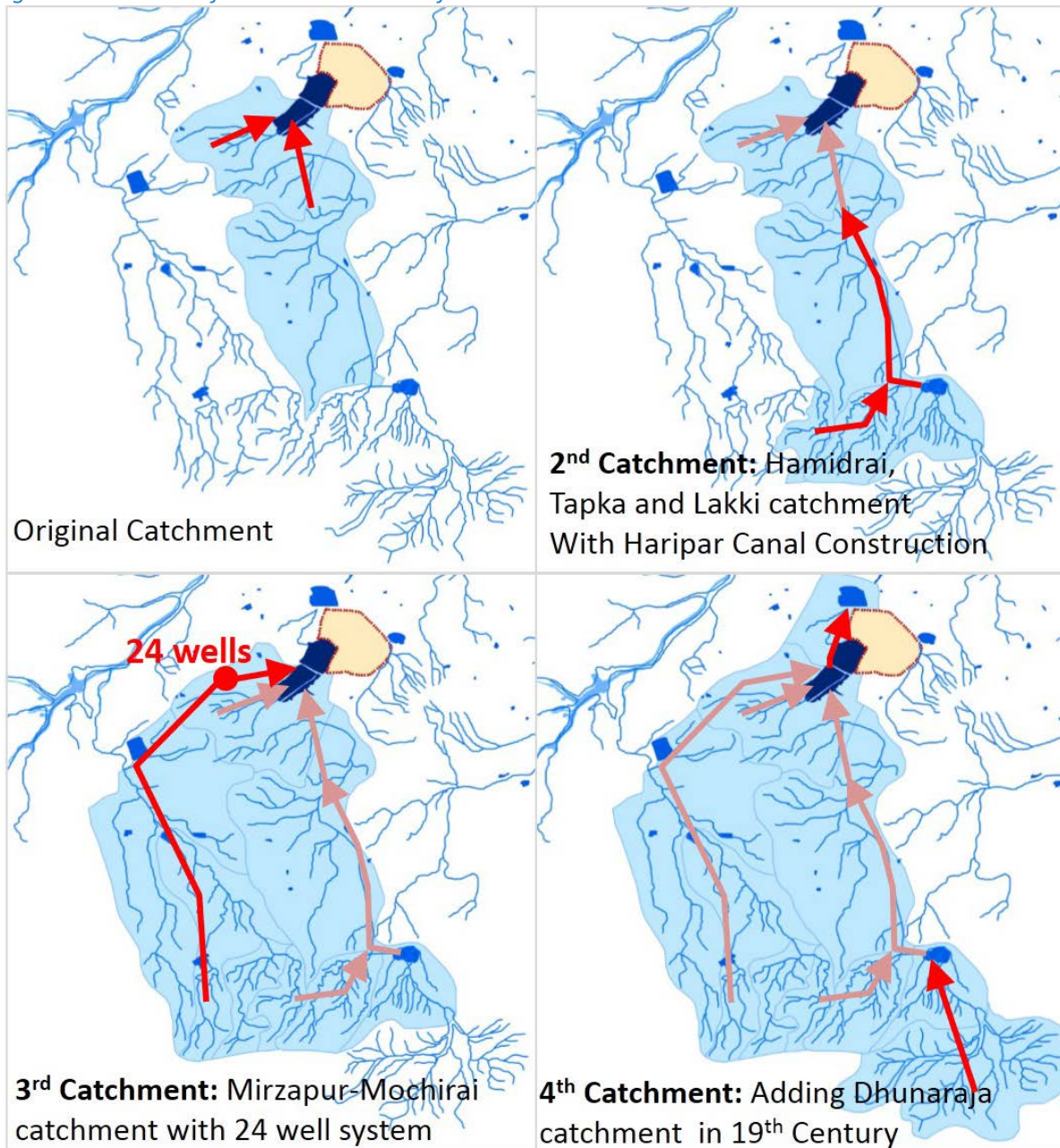
Figure 4: Evolution of linked catchments of Hamirsar
