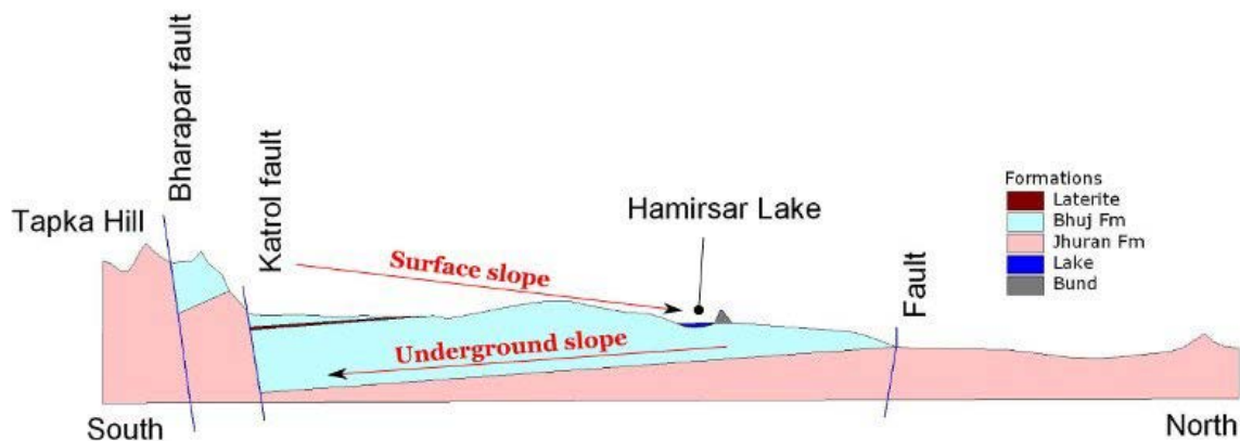
Figure 3: Schematic representation of Bhuj Aquifer
