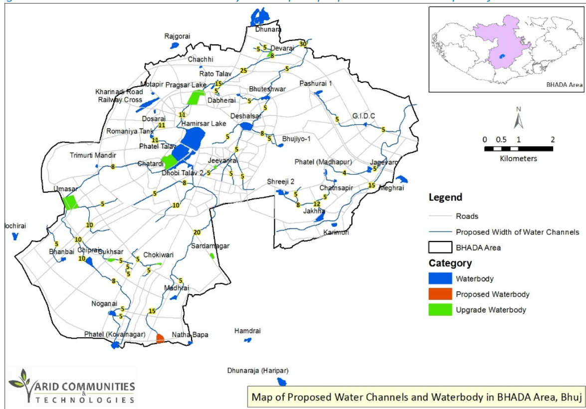
Figure 34: Water channel and water body revival plan proposal submitted as part of DP revision
